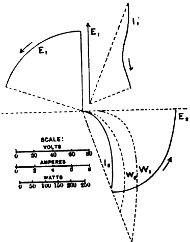
FIG. 20.—Constant Potential, Step Up, Arm at 180^\circ .
